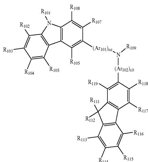
Formula 201
