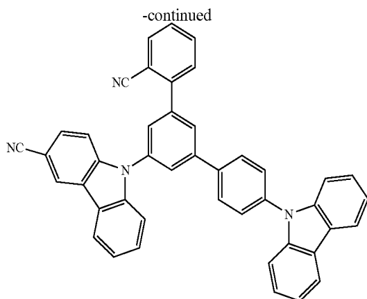
Compound 160
