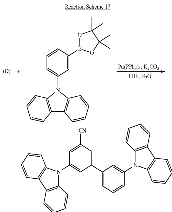
Compound A
