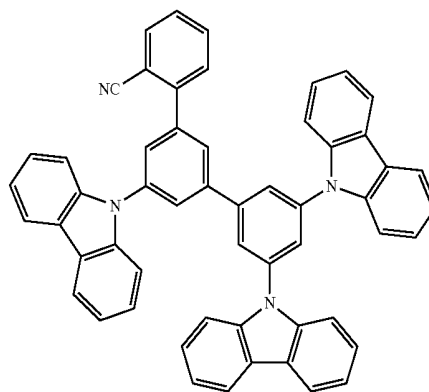
Compound B
