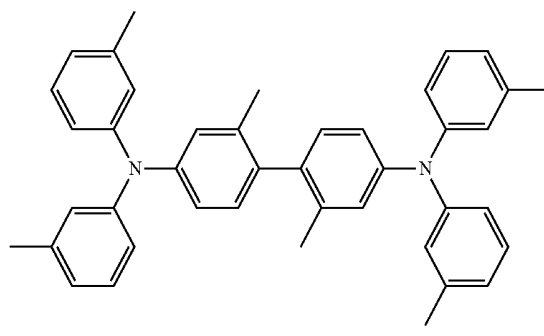
HMTDP
