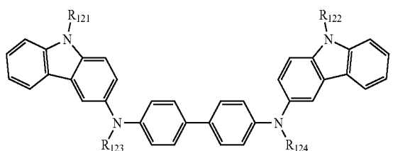
Formula 202
