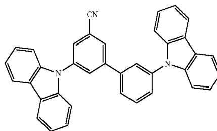
Compound A
