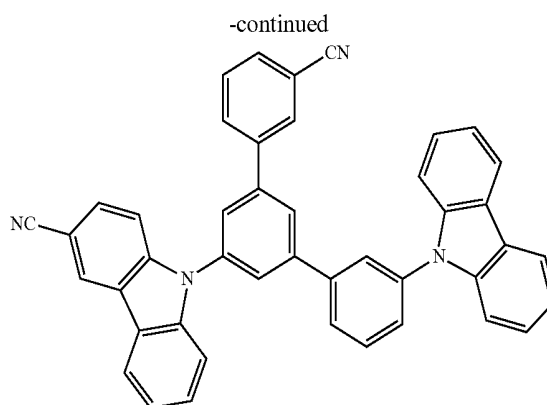
Compound 22
